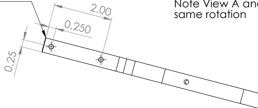
VIEW A SCALE 1 : 2
